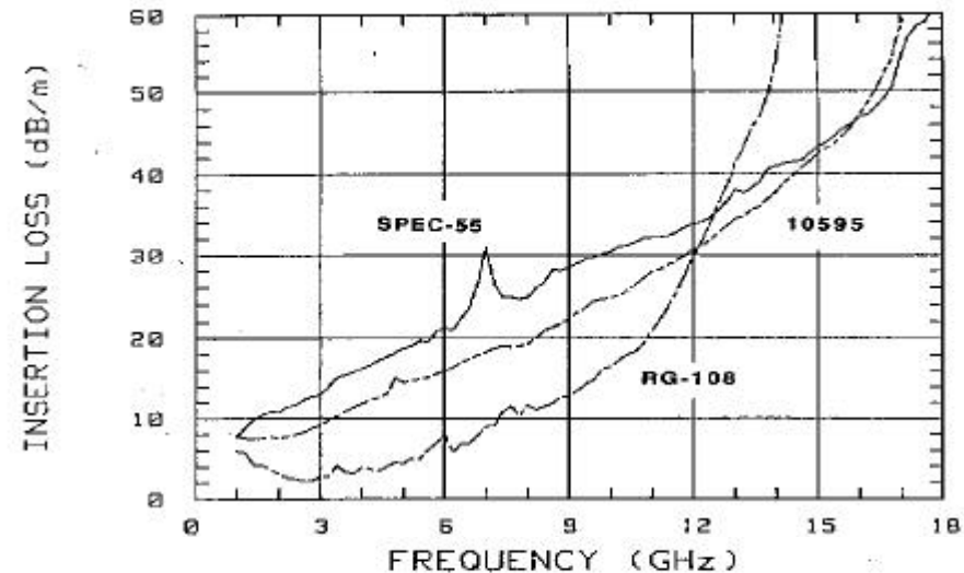
Insertion Loss of Aerospace Cables with Single Braid Shields
