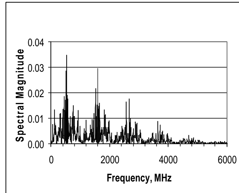
Spectrum of Quasi-Random Pulses
