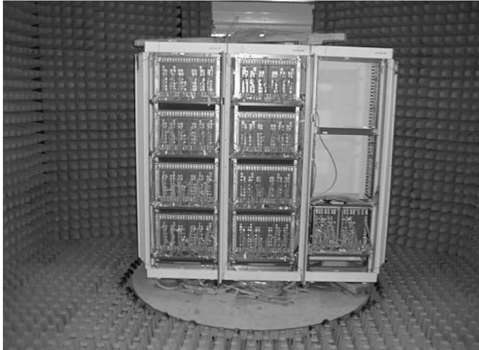
GSS64K Front side with open doors.
